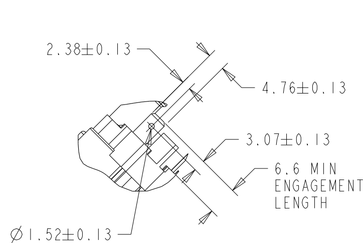
VIEW C
